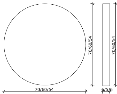
lajeta circular
